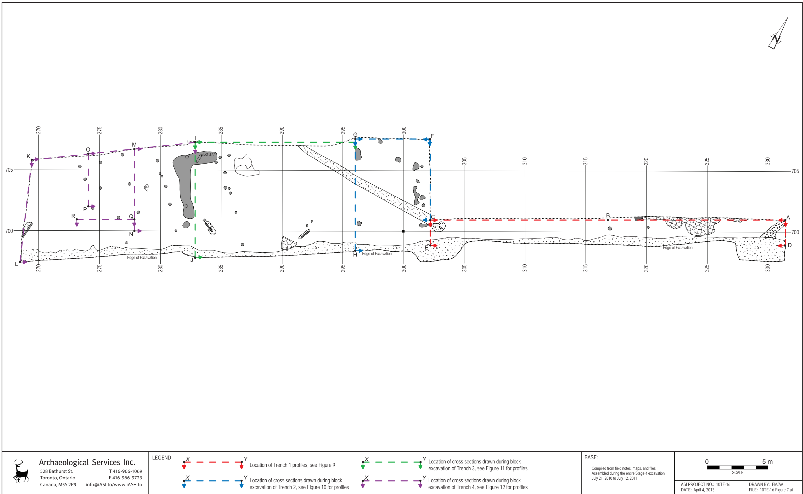
Figure 8: Locations of cross sections drawn during the Stage 4 excavation of the Visitors' Centre at the Fort York National Historic Site (AjGu-26).
