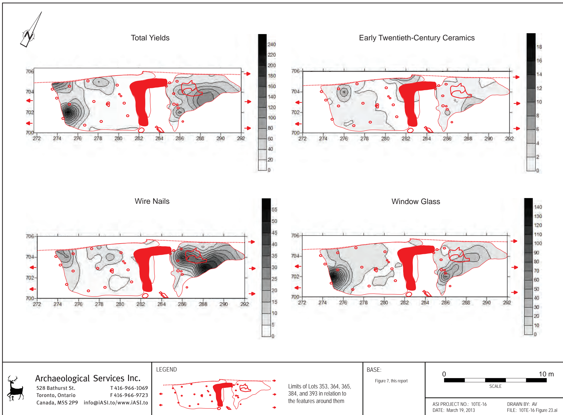
Figure 23: Spatial distribution of major artifact types in Lots 353, 364, 365, 384, and 393, working surfaces of the carpenter shop and forge.
